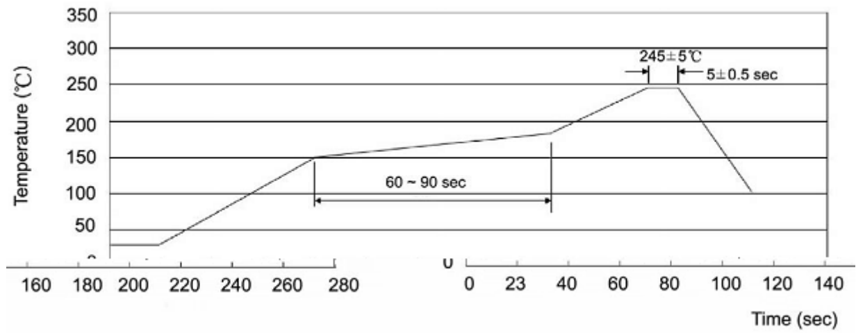
Temperature Profile for IR Reflow Soldering(Pb-Free)
