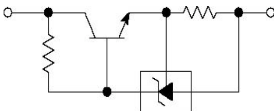
Constant Current Source
