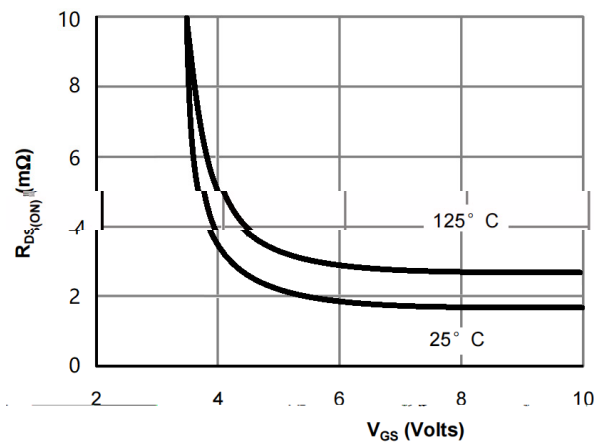
Figure 5: On-Resistance vs. Gate Voltage
