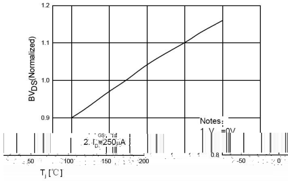
Breakdown Voltage Variation vs. Temperature
