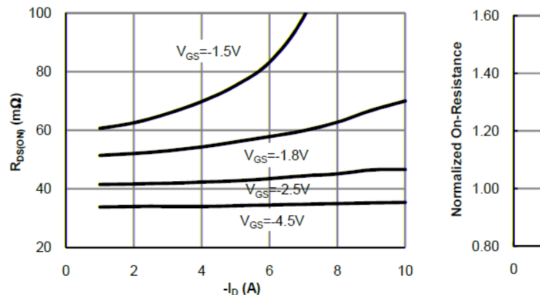
Figure 3: On-Resistance vs. Drain Current and Gate Voltage (Note E)
