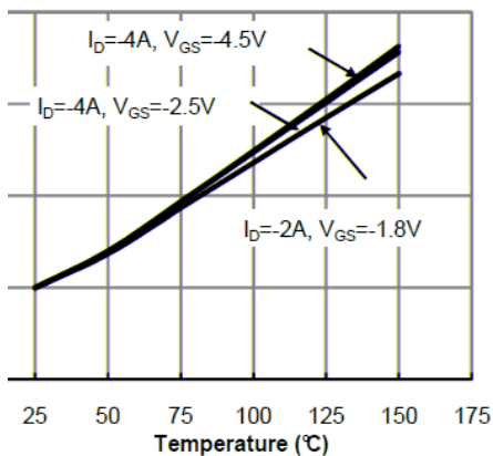
Figure 4: On-Resistance vs. Junction Temperature (Note E)
