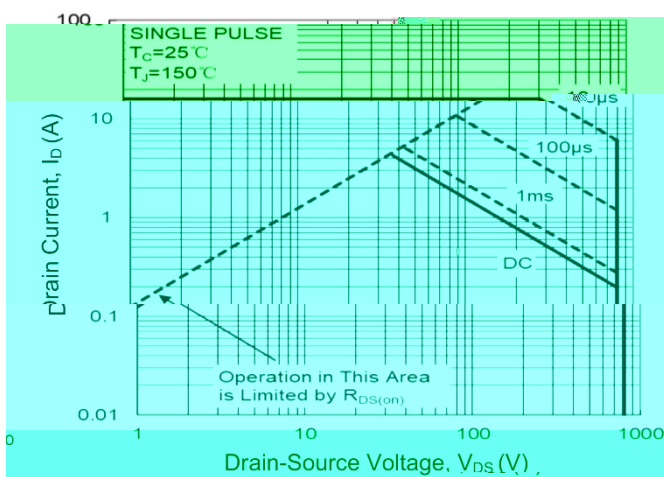
5. Safe Operating Area (SOA)
