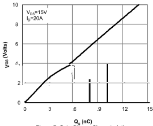
Figure 7: Charge Characteristics
