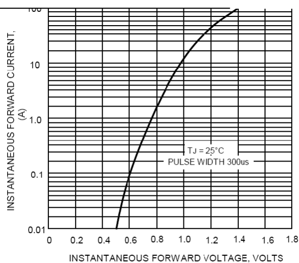
FIG.4-TYPICAL FORWARD CHARACTERISTICS
