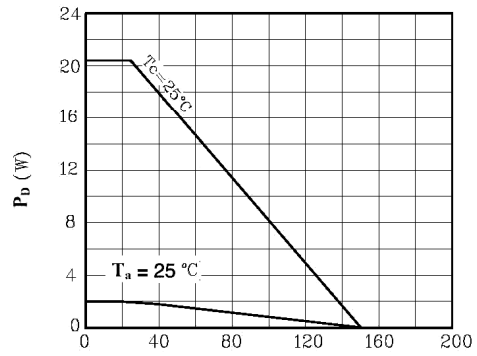
P_D - T_a
