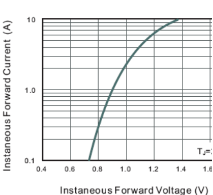
Fig.3 Typical Forward Characteristic
