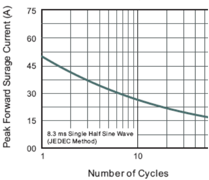
Fig.5 Maximum Non-Repetitive Peak Forward Surge Current
