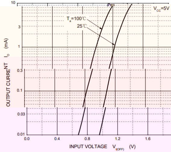
Figure 2: OFF Characteristics
