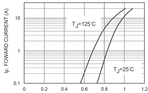
FIG.4-TYPICAL FORWARD CHARACTERISTICS
