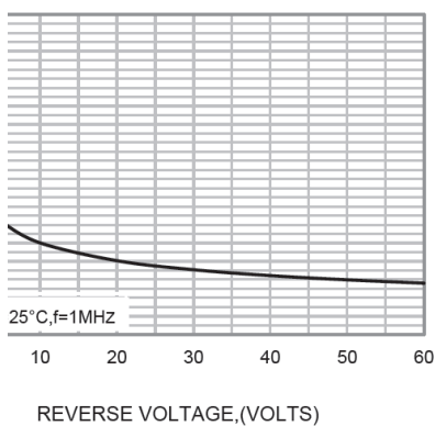
FIG.3-TYPICAL JUNCTION CAPACITANCE
