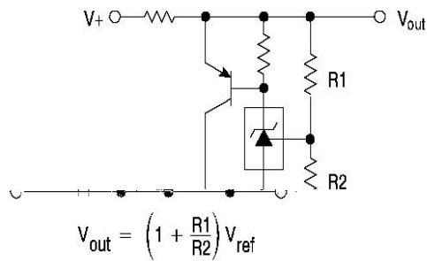
Higher-current Shunt
