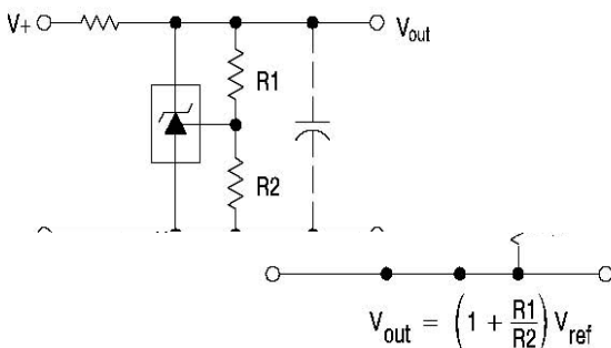
Shutdown Regulator
