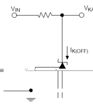
Test Circuit For I_{KA(OFF)}
